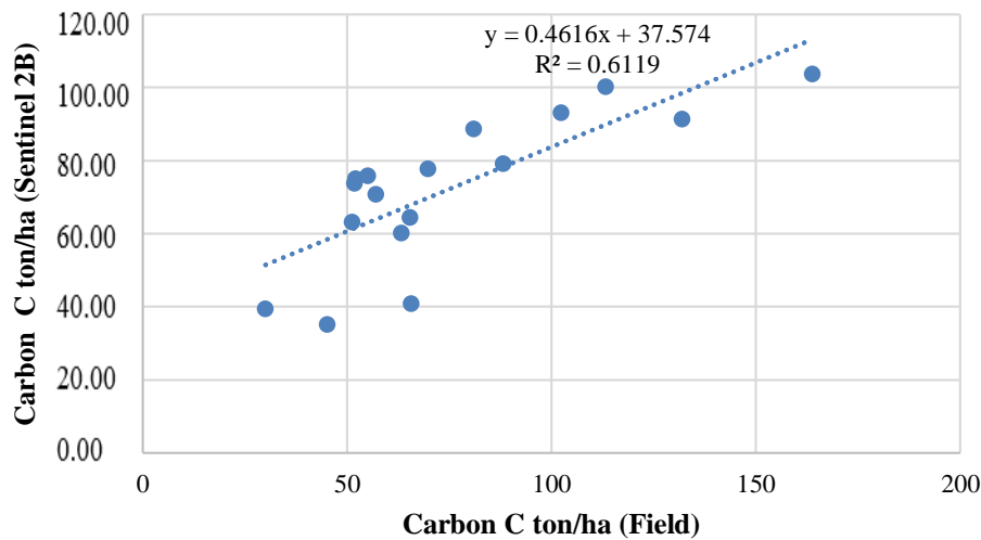
Figure 8. Regression function between measured and image-predicted carbon
