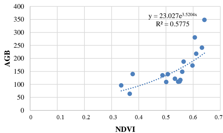
Figure 5. Correlation between AGB and NDVI models
